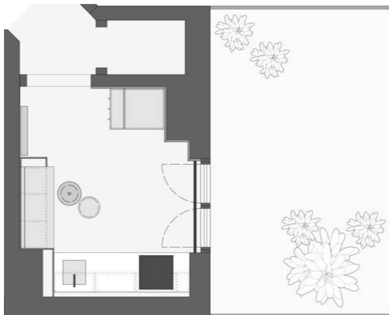
Grundriss • Floor plan
